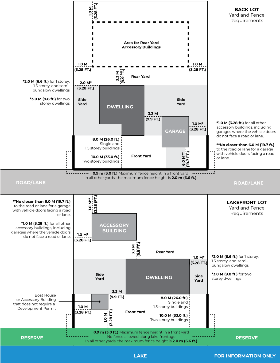
Figure 11: Yard and Fence Requirements
