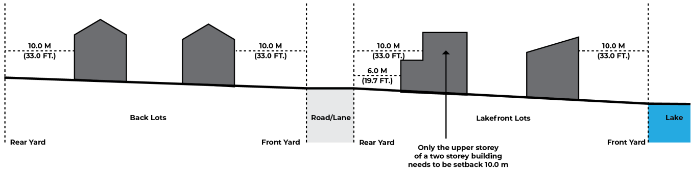
Figure 12: Setbacks for Dwellings
