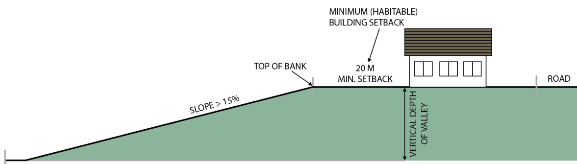
Figure 3 – Setback Requirements
