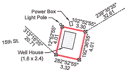
DETAIL Scale 1:250
