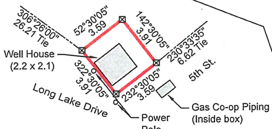
DETAIL Scale 1:250
