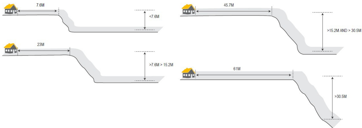
Figure 9.1: Setbacks
