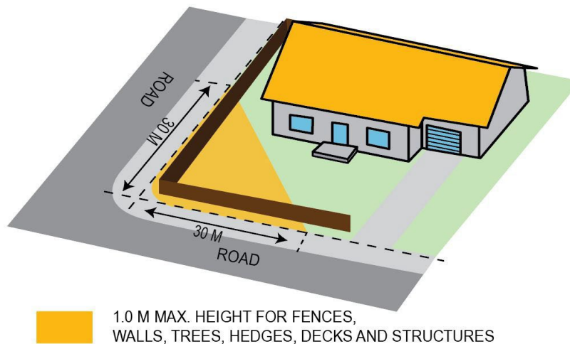
Figure 9.5: Corner Lot Restrictions
