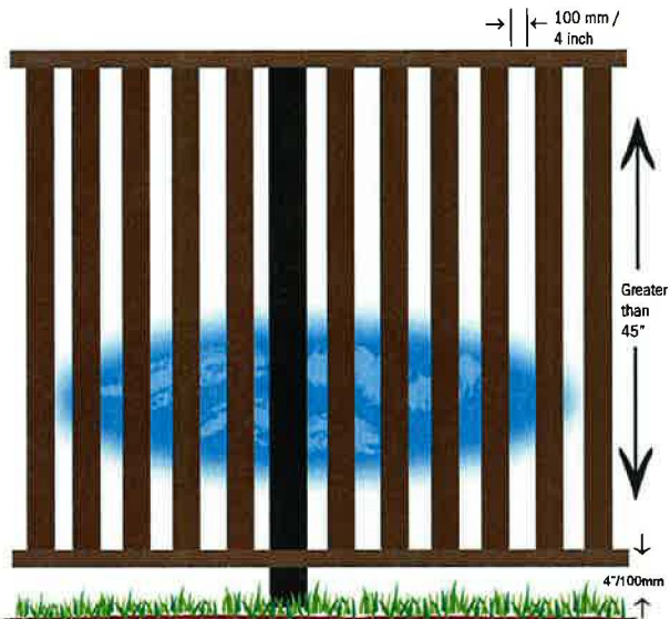
Figure 5: Vertical and horizontal member spacing and ground
