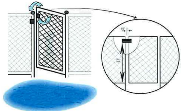
Figure 7: Self-closing and self-latching gate installation
