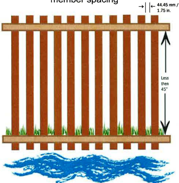
Figure 6: Vertical and horizontal member spacing
