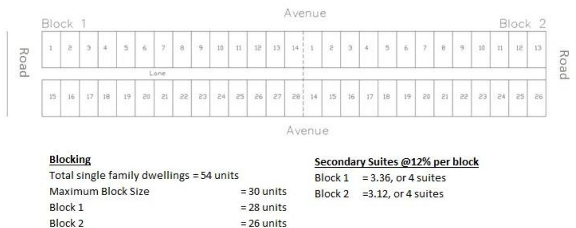
FIGURE 9.6: TYPICAL BLOCKING (SINGLE DETACHED NEIGHBOURHOOD WITH LANE)
