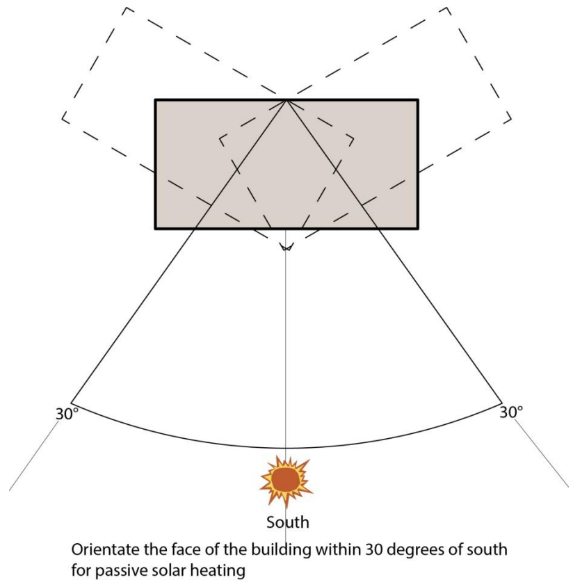
FIGURE 11.1: BUILDING ORIENTATION TO MAXIMIZE SUNLIGHT
