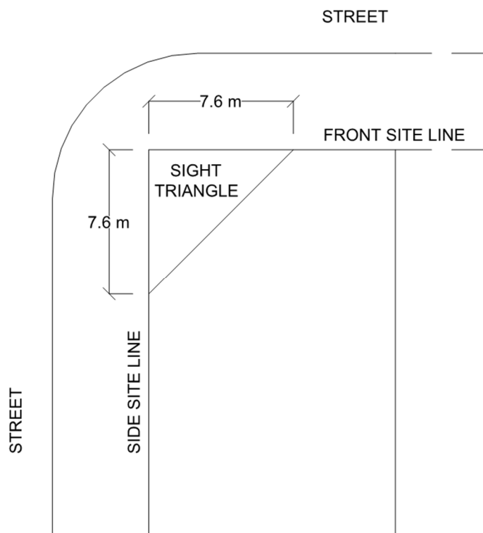
Figure 2-2: Sight Triangle
