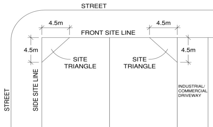
Figure 2-1: Sight Triangles
