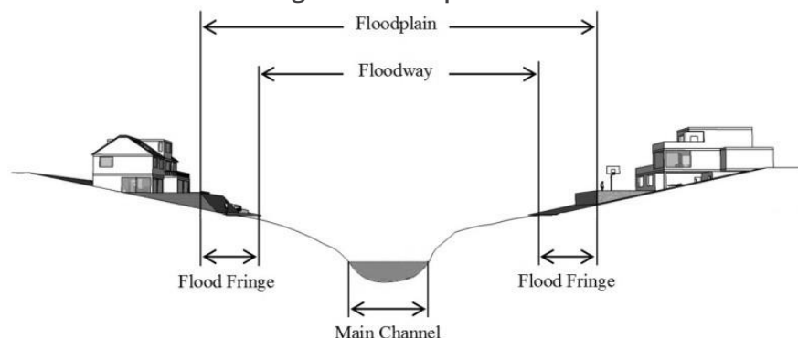
FIGURE 8: Cross-Section of a Flood Fringe And Floodplain
