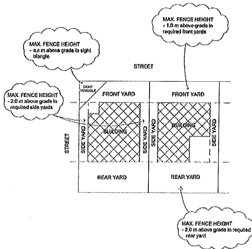
Figure 4-1: Fence Requirements
