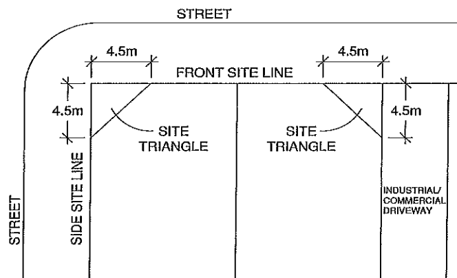
Figure 2-1: Sight Triangles
