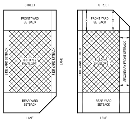
Figure 4.1: Corner Cut-off Lot Minimum Yard Dimensions
