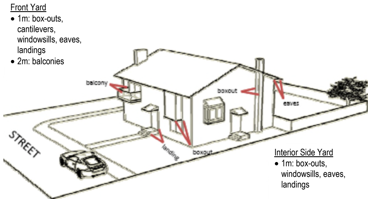
Figure 57-1: Permitted Projections – Front and Interior Side Yard Setbacks
