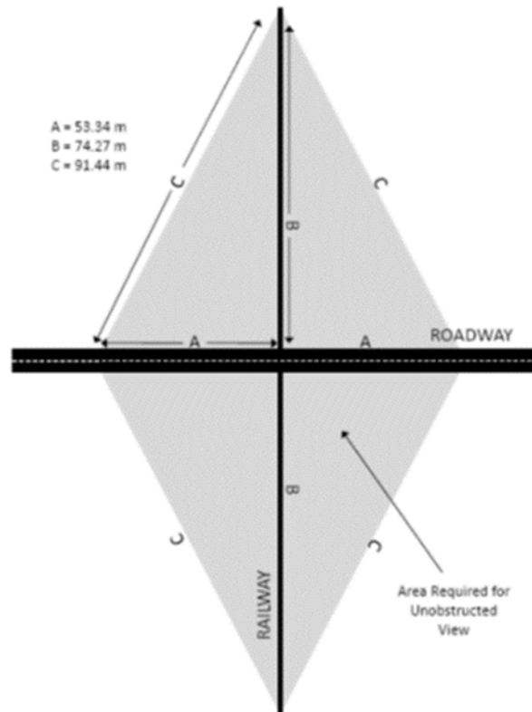
Figure 64-2: Sight Triangle at Road and Rail Intersections
