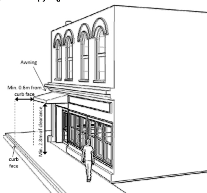
Figure 69-1: Awning and Canopy Signs
