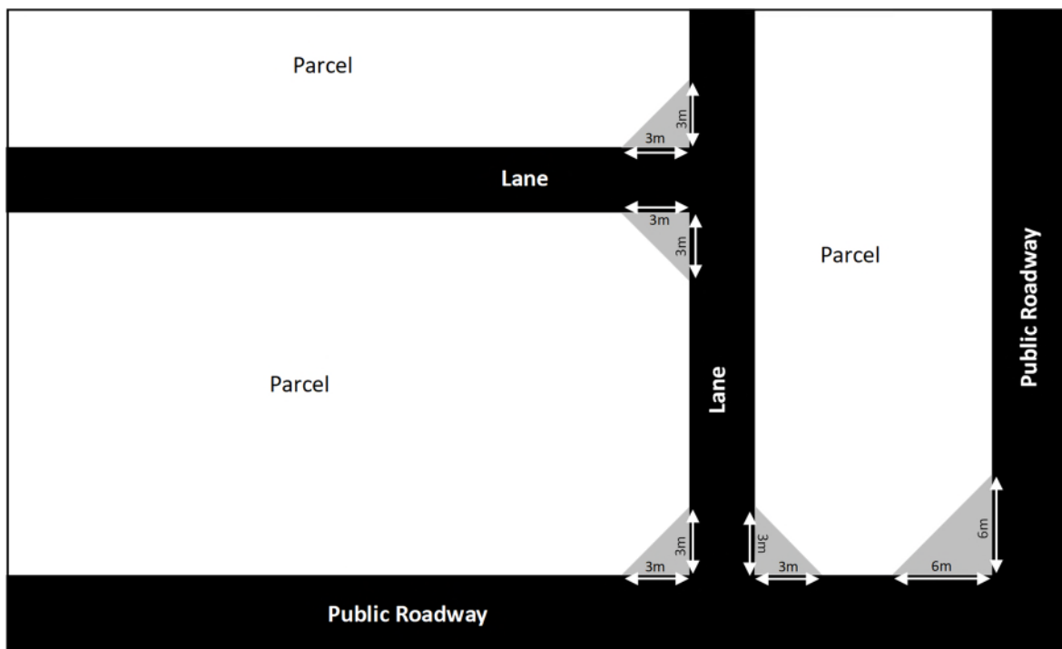
Figure 64-1: Sight Triangle at Intersections
