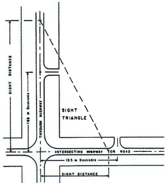
Figure 3: Sight Triangle Diagram (Source: Government of Saskatchewan)
