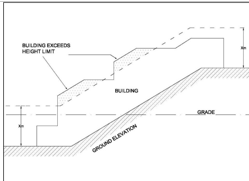
Figure 12: Building Height
