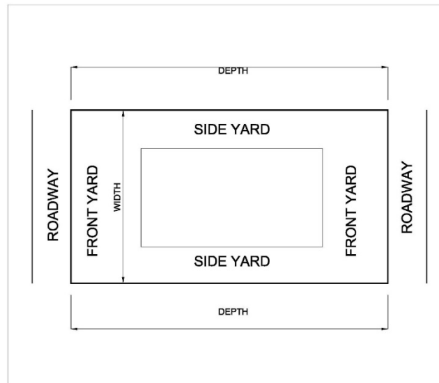
Figure 14: Double Fronting Lot
