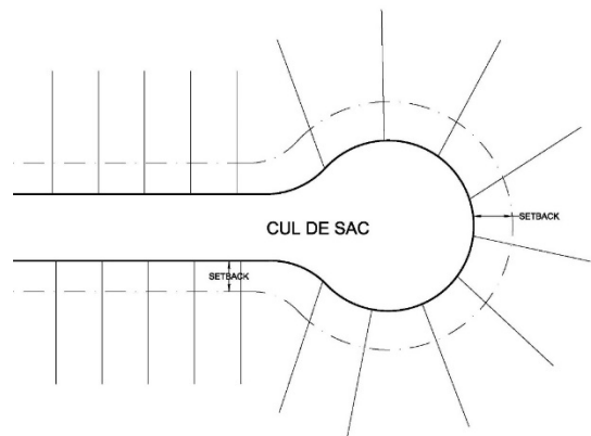
Figure 16: Setback Definition Diagram B
