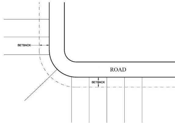
Figure 15: Setback Definition Diagram A
